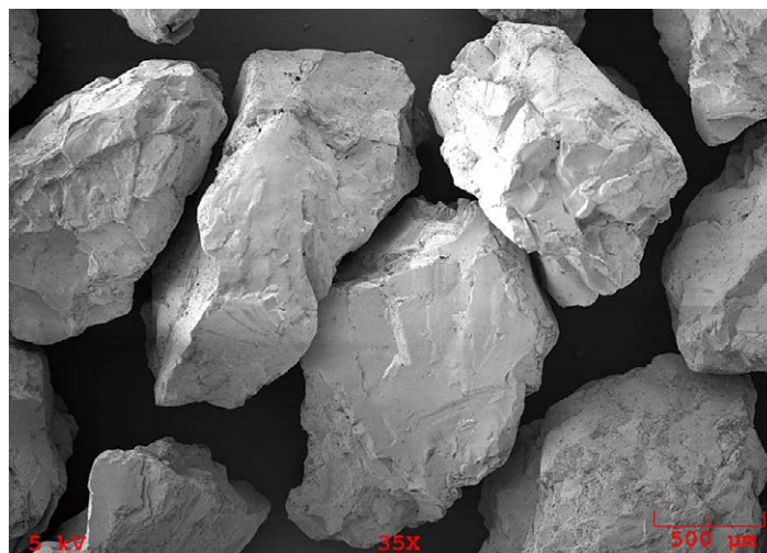
SEM Photomicrograph of Metcolite C, showing blocky, sharp-edged particle morphology.
